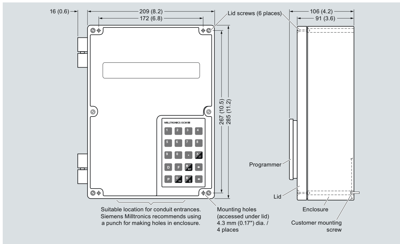
OCM III, dimensions in mm (inch)
