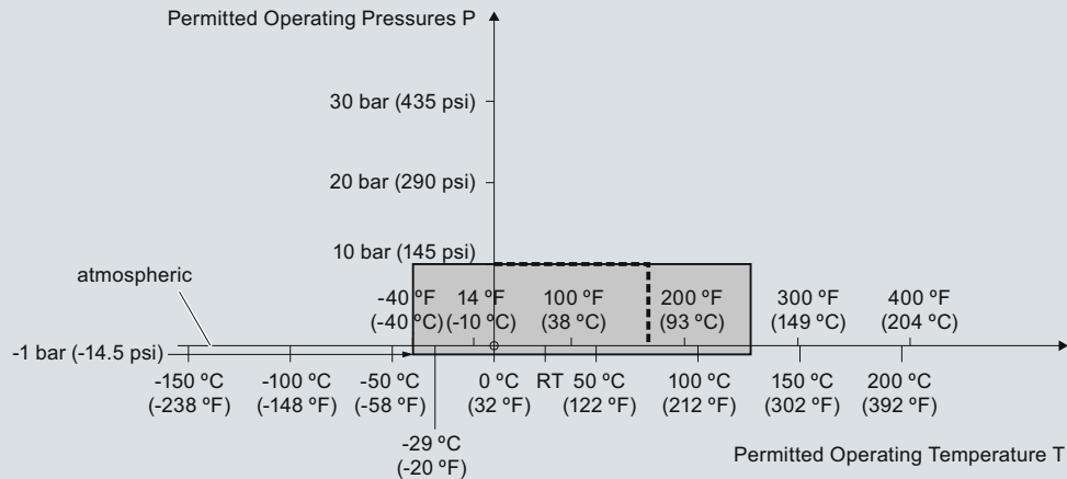
Pressure/Temperature Curve CLS200 Sliding Coupling Threaded Process Connections (7ML5633 and 7ML5643)
