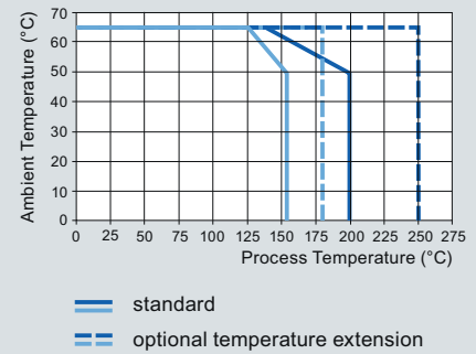
SITRANS LR400
