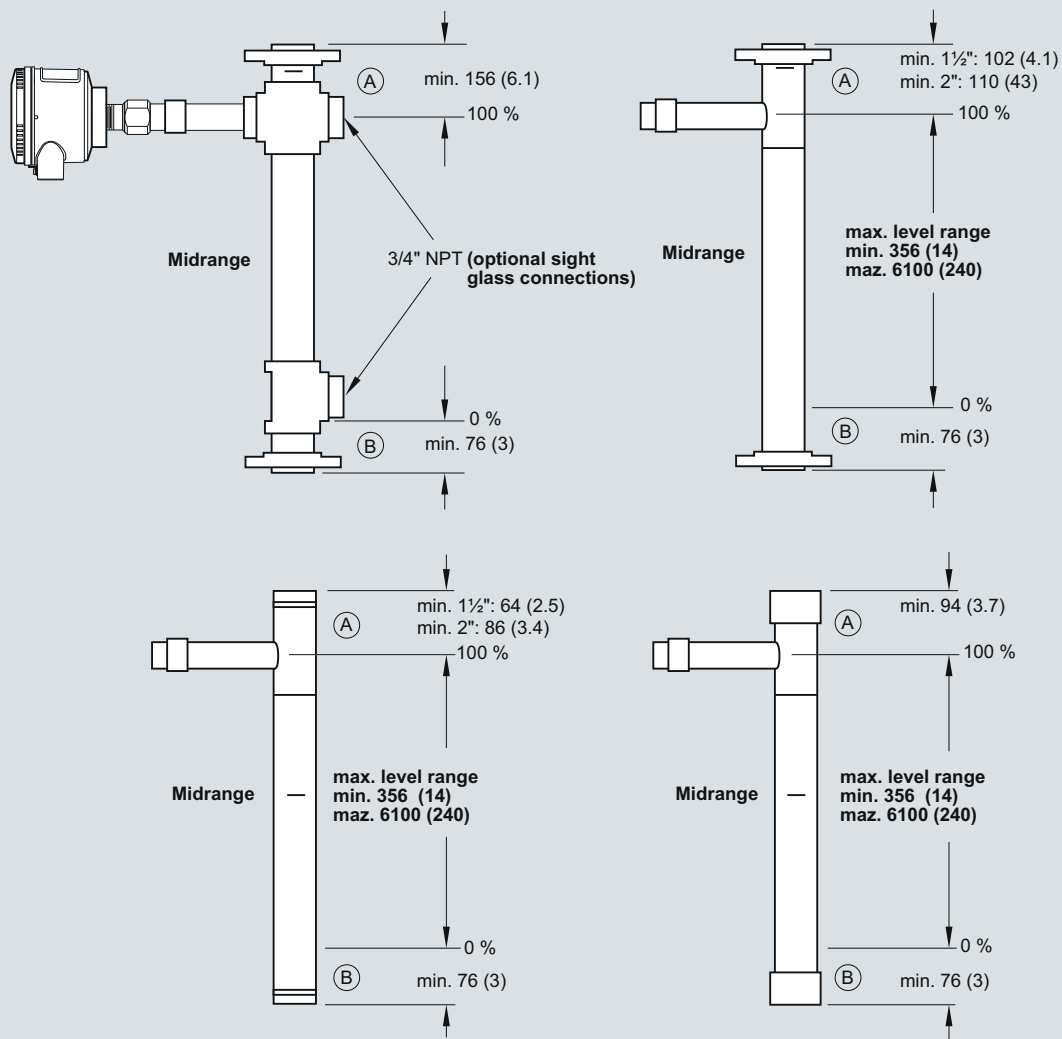
SITRANS LG200 - Model 7ML1305-1 Chamber Replacement Probe, dimensions in mm (inch)
