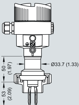
Bolting DN40
