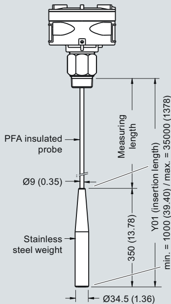
Cable version, insulated welded flange (7ML5513)
