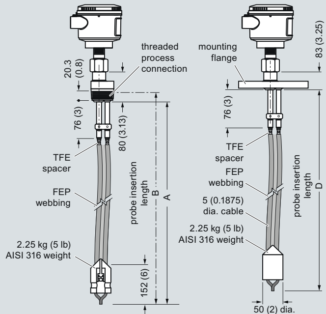
7ML1302-2 (7x5-x) Twin Rod Bulk Solids Flexible Probe Threaded or Flanged Connection
