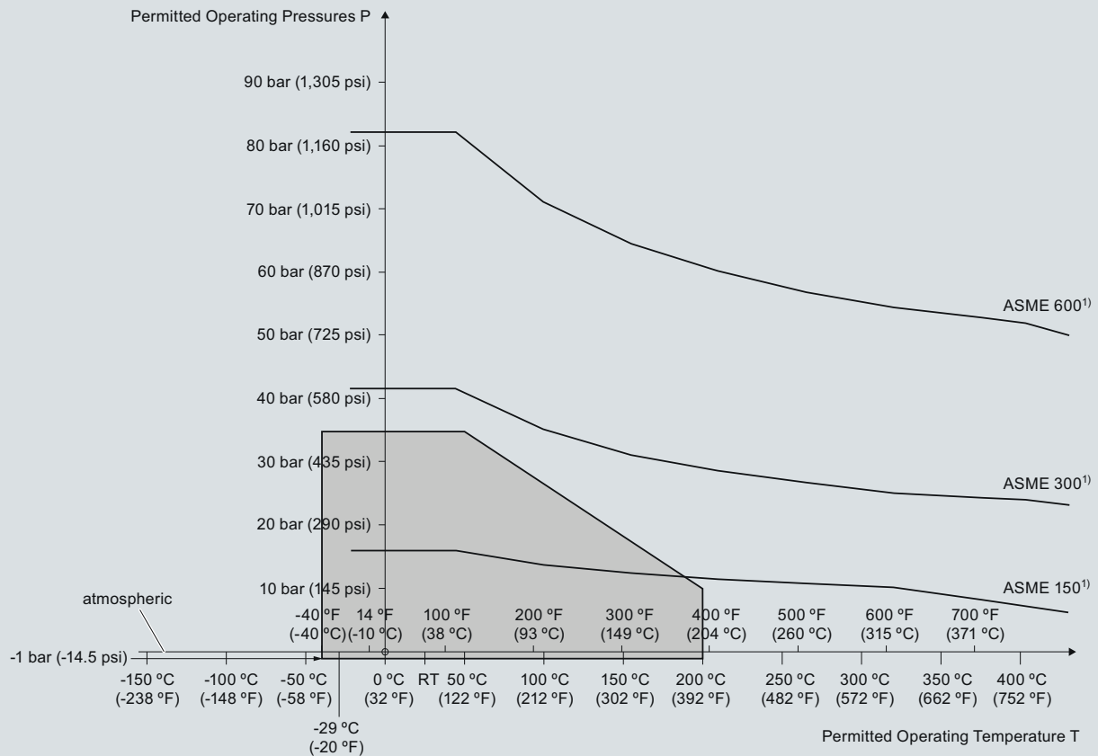
Pressure/Temperature Curve LC300 Standard, Extended Rod and Cable Probes ASME Flanged Process Connections (7ML5670, 7ML5671, 7ML5672 and 7ML5673)
