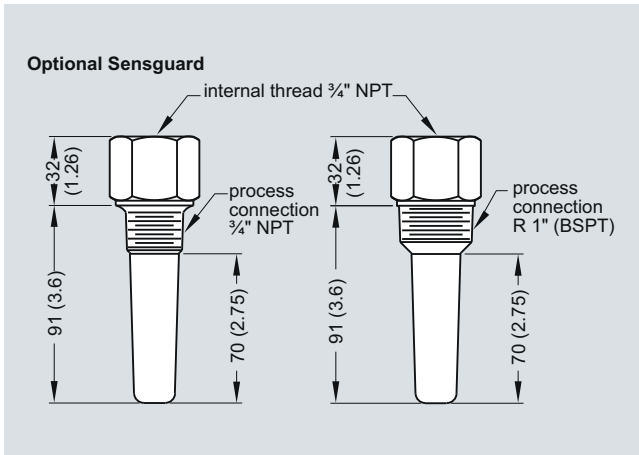
Optional Sensguard, dimensions in mm (inch)
