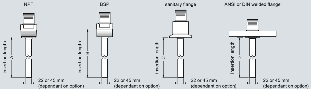
Probe Connections and Insertion Lengths (Note BSP connections differ from NPT)
