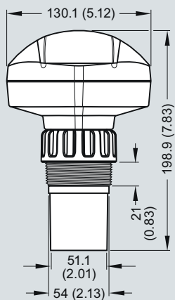
SITRANS Probe LU, dimensions in mm (inch)
