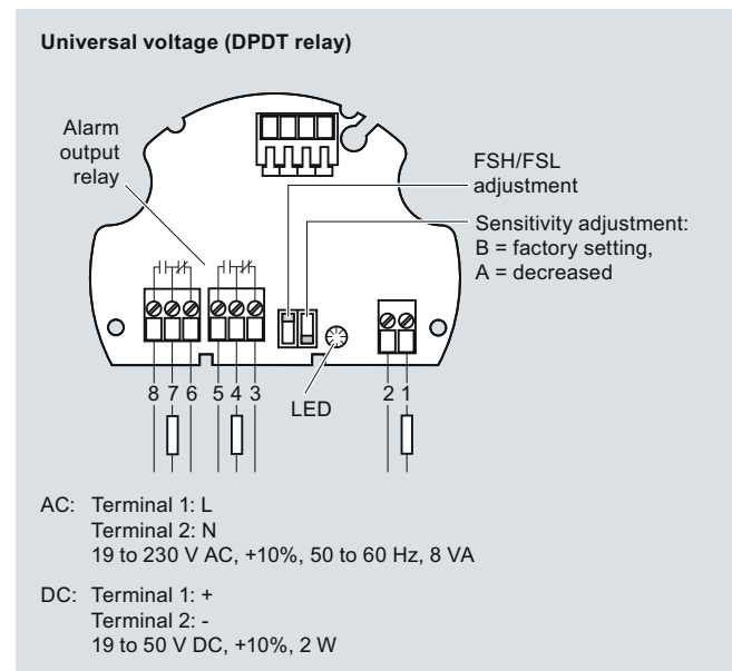
Schematics
