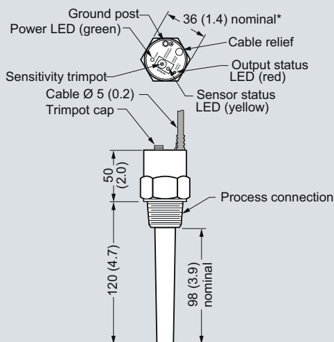
Pointek CLS100 dimensions, dimensions in mm (inch)
