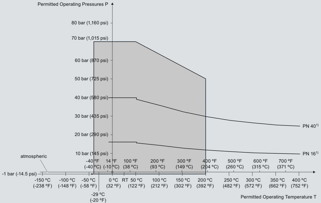
Pressure/Temperature Curve LC500 Single Piece Flanged Rod Probes with PTFE facing EN Flanged Process Connections (7ML5517)
