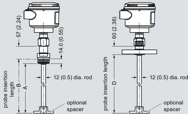
7ML1303-1 (7xF-x) Probe, Threaded and Flanged Connection
